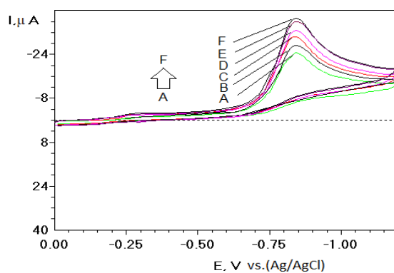
Figure 6: Cyclic voltammograms of Pioglitazone Hydrochloride at different scan rate (40 to 90 mV/s) in HCl. We draw the curve that represents the changes of the values of current I_p ( \mu\text{A} ) with square root of scan rate \sqrt{V} as shown in (Fig.7).
