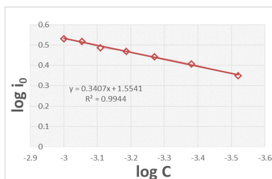
Figure 4: Graph of \log(i_0) of \log(C) in HCl.
