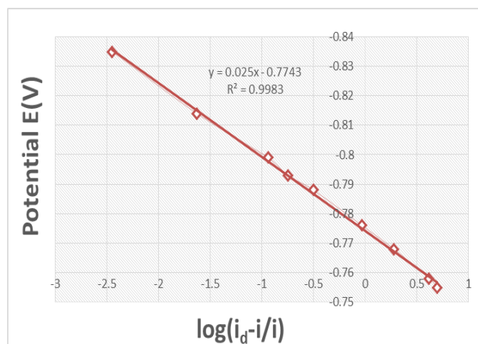
Figure 5: Graph of E(V) of \log(i_d-i/i) in HCl.
