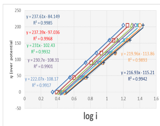
Figure 3: Graph of \eta of \log(i) for different concentrations of Pioglitazone Hydrochloride.
