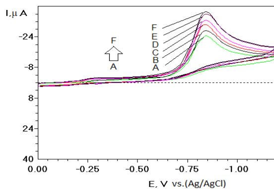
Figure 6: Cyclic voltammograms of Pioglitazone Hydrochloride at different scan rate (40 to 90 mV/s) in HCl. We draw the curve that represents the changes of the values of current I_p ( \mu A ) with square root of scan rate \sqrt{V} as shown in (Fig.7).
