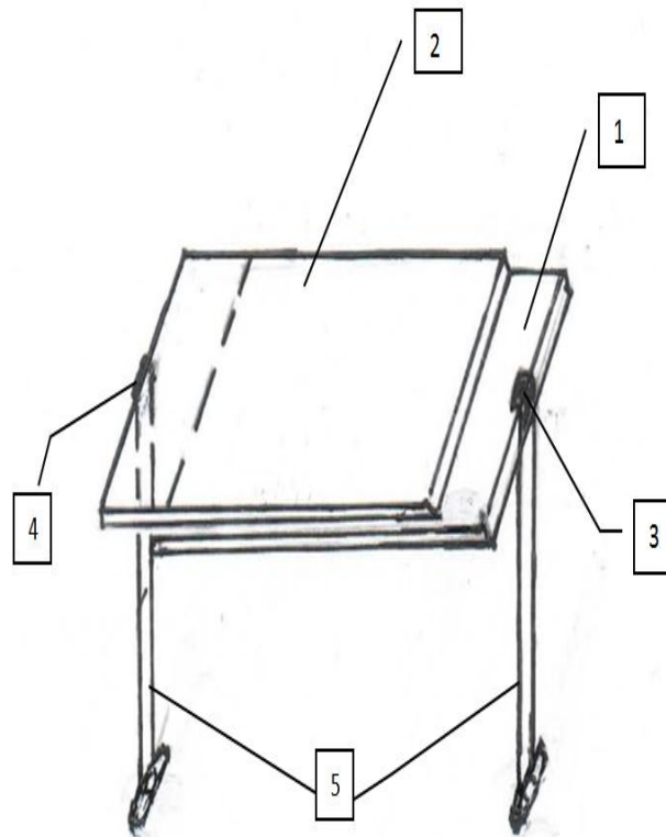
Fig. 7: Mininanoscope sensor for supramolecular information exchange between the integral organism and biosphere on the skin surface.
