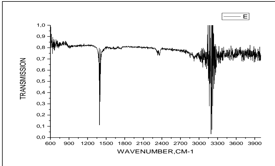
Fig. 8: Spectral image of the uniform "superperfect energy" recorded with mininanoscope sensor.
